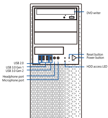
Front View NC5406T-HD
