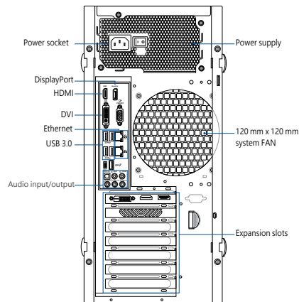
Rear View NC5406T-HD
