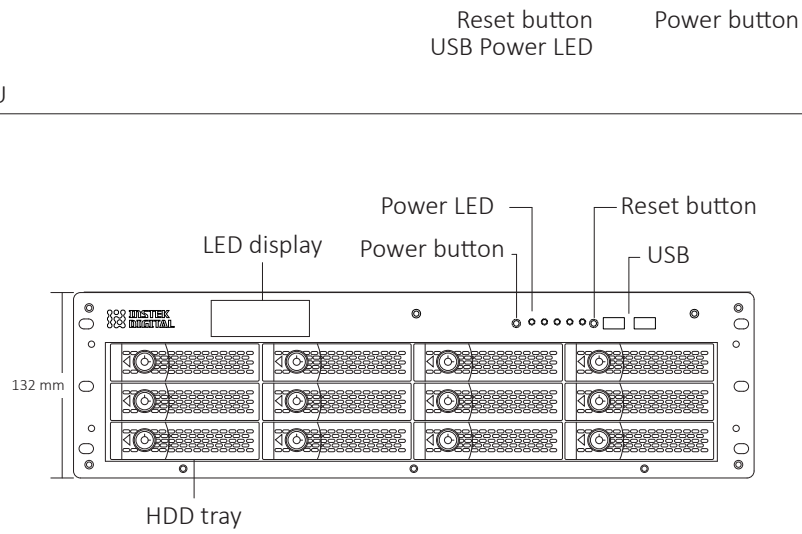
Front View ID-NR5400-3U
