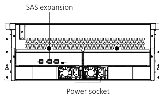
Rear View | DS2316-JB
